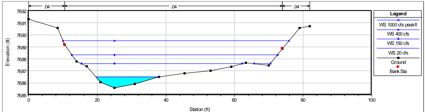
Freestone Aquatics Post Construction - Note the thalweg definition and existing low flow channel
