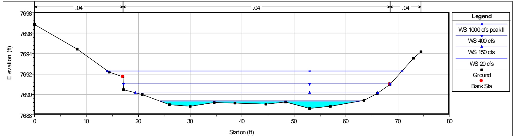
Freestone Aquatics Pre Construction - Note the lack of thalweg definition and no low flow channel
